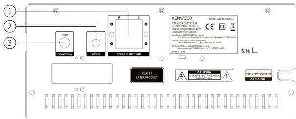
Backside
